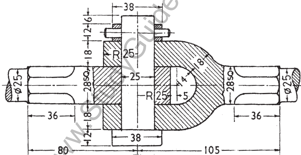
PIN-JOINT OR KNUCKLE JOINT
